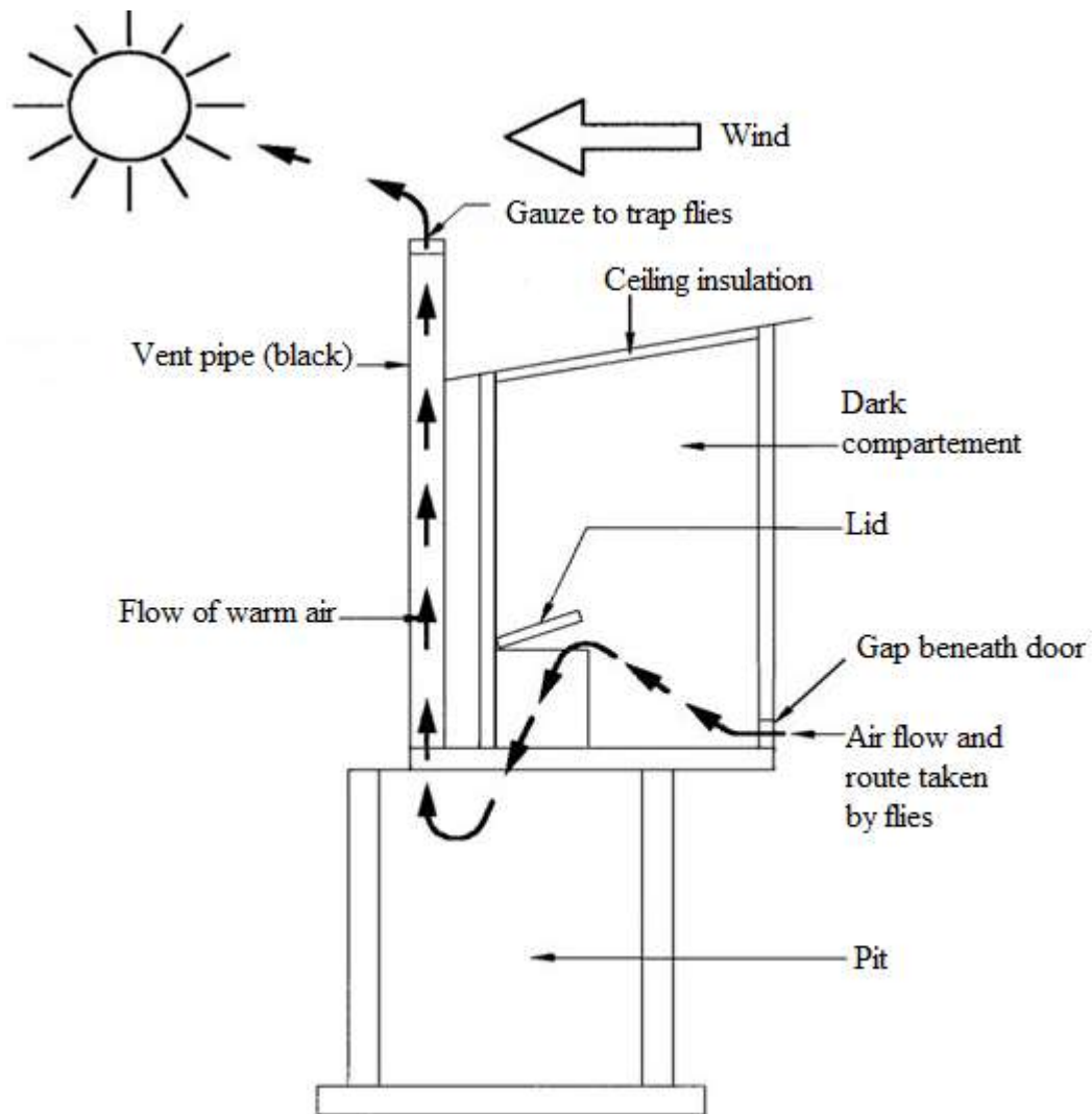
Figure 4.11.12-2 The Concept behind Ventilated Improve Pit latrines
