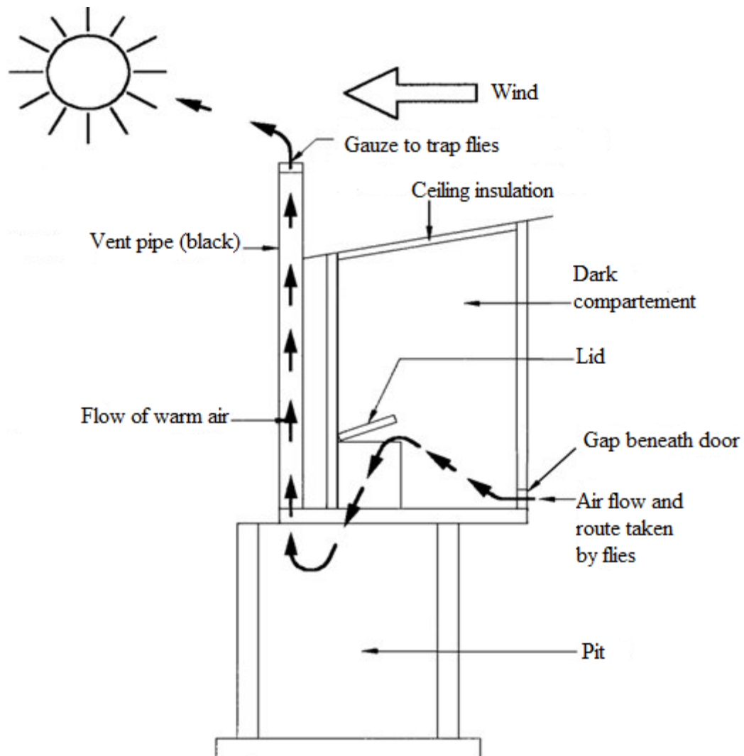
Figure 4.11.12-2 The Concept behind Ventilated Improved Pit Latrines
