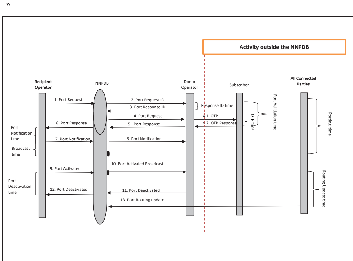
Figure 11: Port Request, Port validation and Activation"
